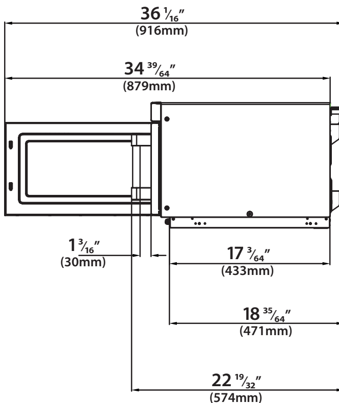
SIDE VIEW (DOOR OPEN)
