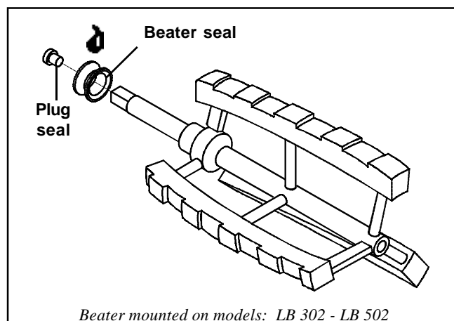
Beater mounted on models: LB 302 - LB 502
