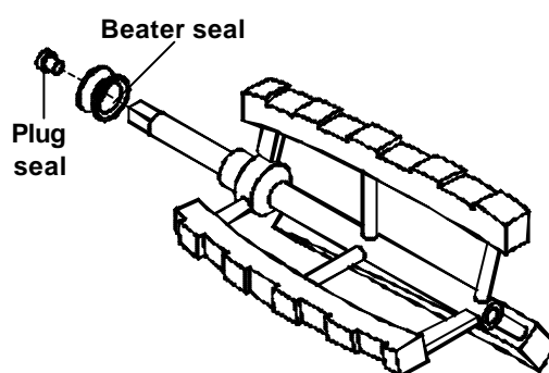
Beater mounted on models: LB 302 - LB 502
